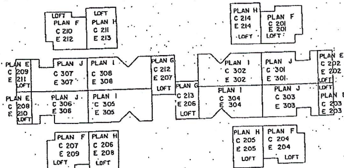
THIRD LEVEL
